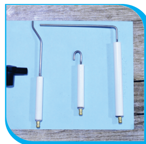
ELECTRODE SENSOR
